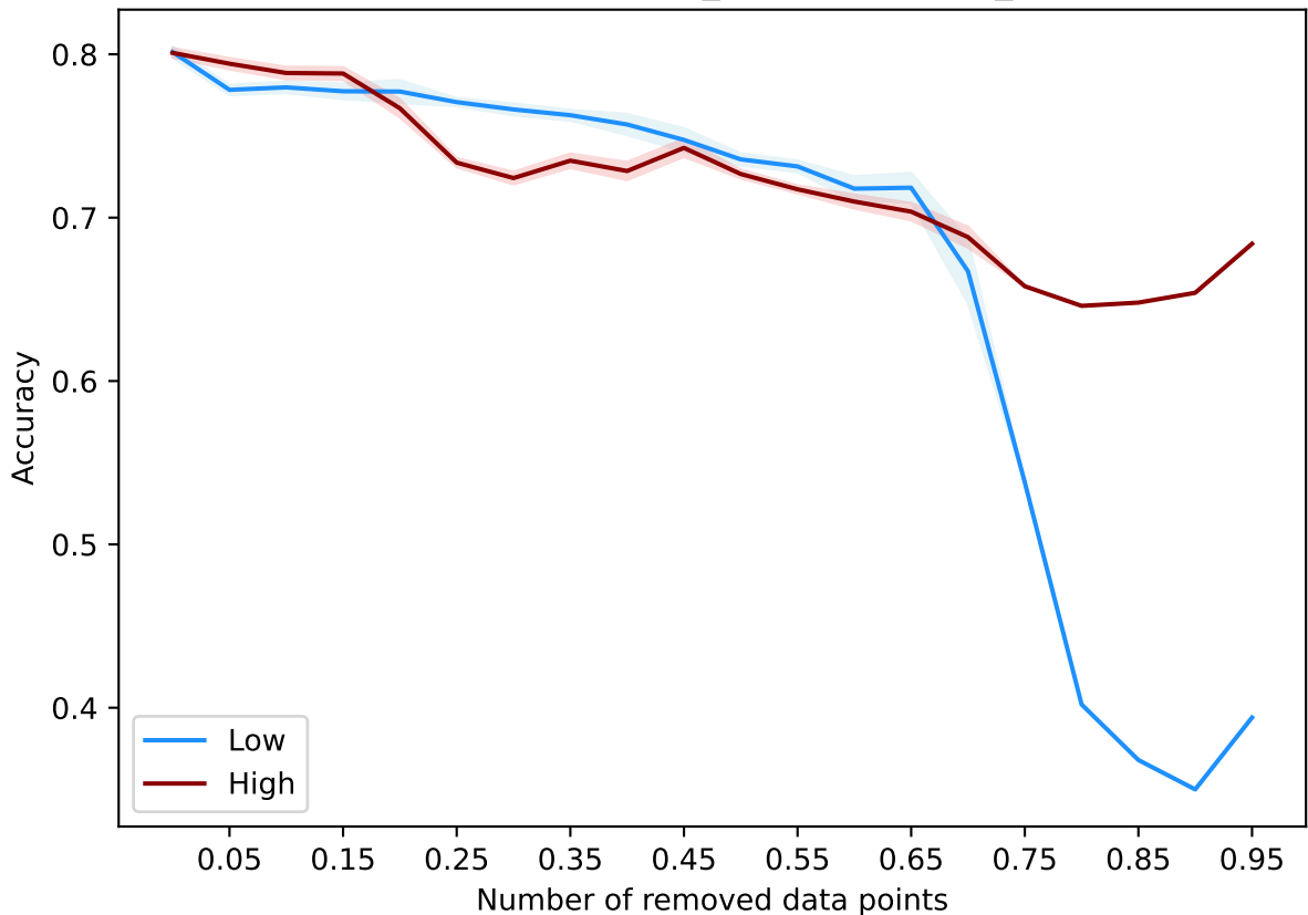
PruningOptimization(optimization_type=size, only_size=150) - adult
